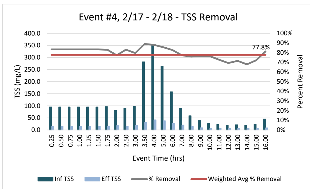
Figure 34: Event #4 influent and effluent TSS lab data.
