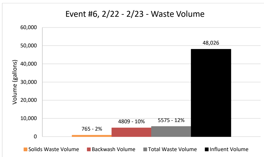
Figure 44: Event #6 waste volumes as a percentage of forward flow.
