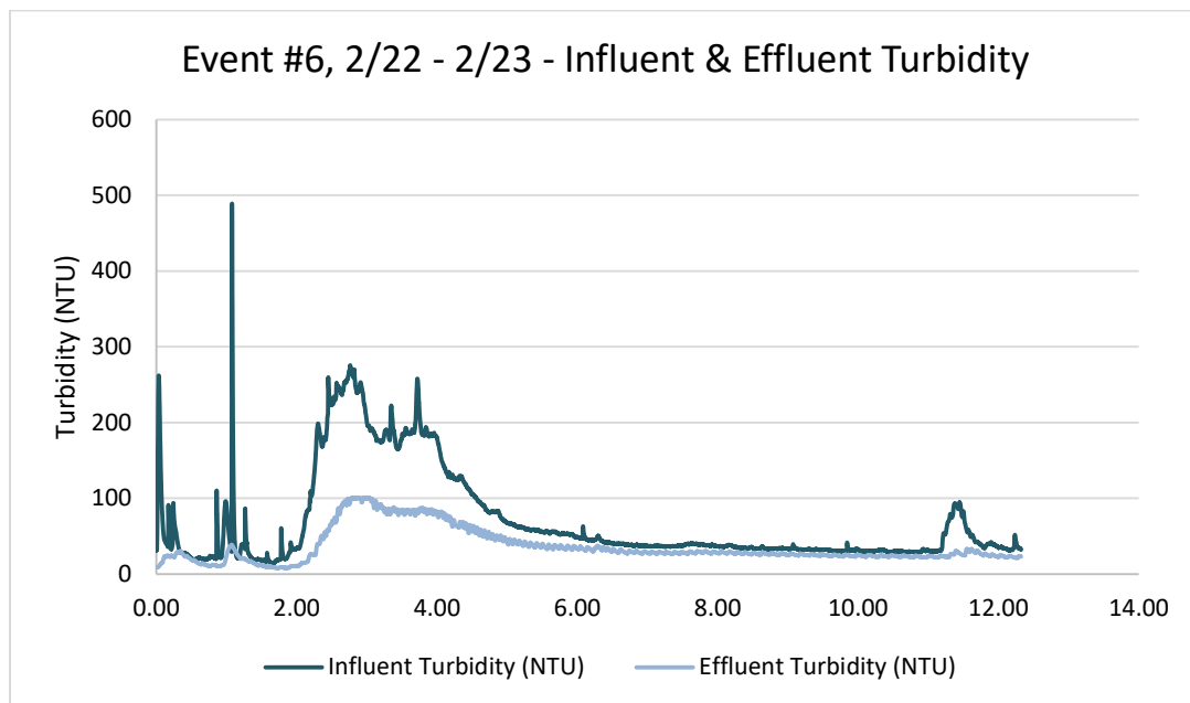
Figure 41: Wet weather event #6 turbidity performance per SCADA data.
