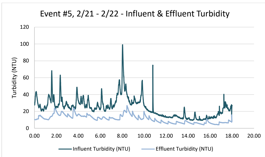
Figure 37: Wet weather event #5 turbidity performance per SCADA data.
