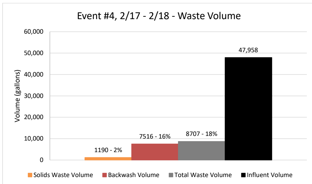
Figure 36: Event #4 waste volumes as a percentage of forward flow.
